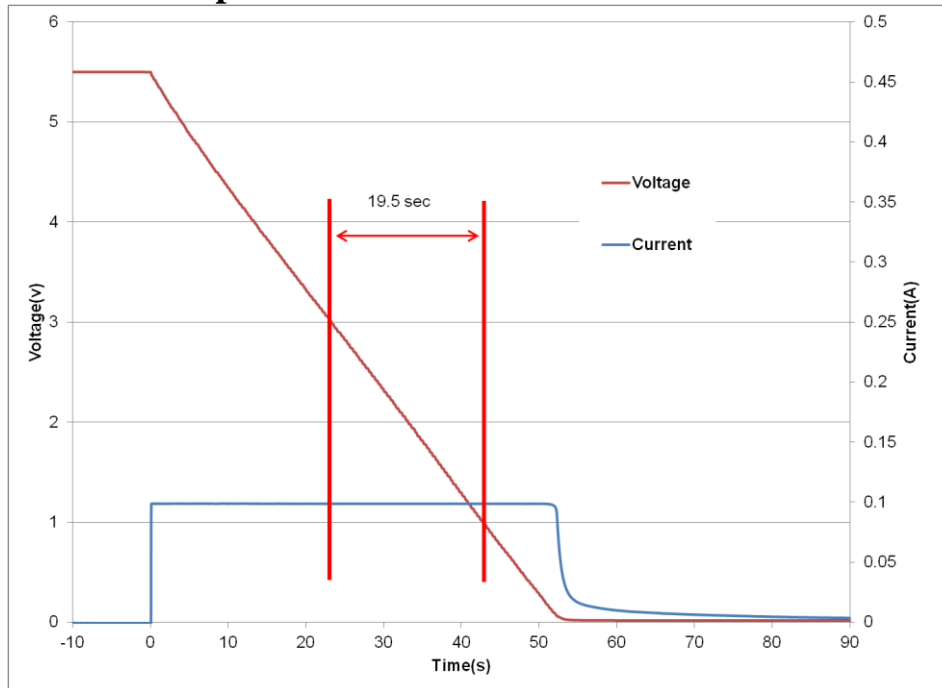
Fig 2: Measurement of DC Capacitance for an HS208
