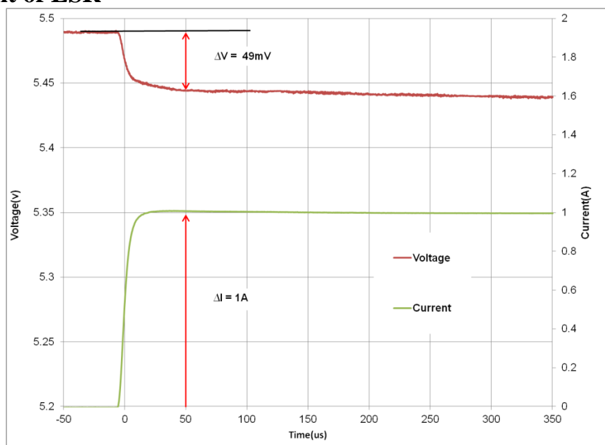
Fig 3: Measurement of ESR for an HS208
