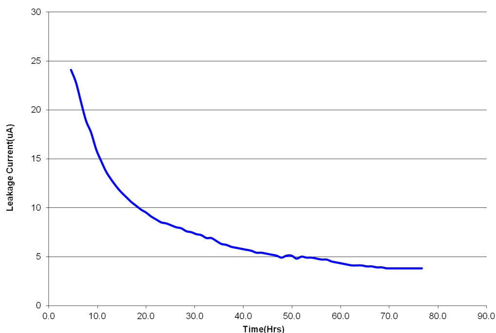
Fig 10: Leakage Current
