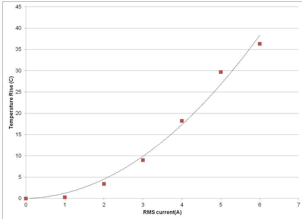
Fig 12: Temperature rise in HS208 with RMS current
