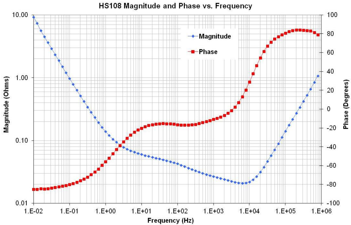
Fig 8: Frequency Response of Impedance (biased at 2.5V with a 50mV test signal)
