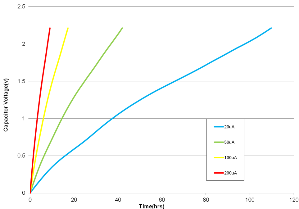
Fig 11: Charging an HS108 with low current
