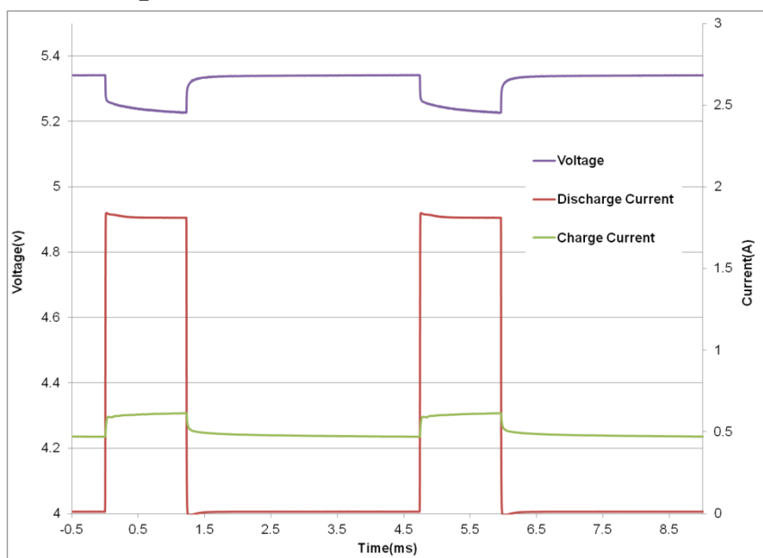
Fig 5: HS208 Pulse Response with GPRS Class 10 Pulse Train
