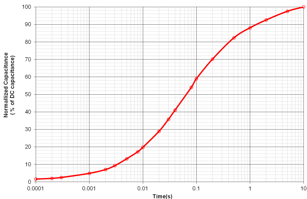
Figure 4: Effective Capacitance
